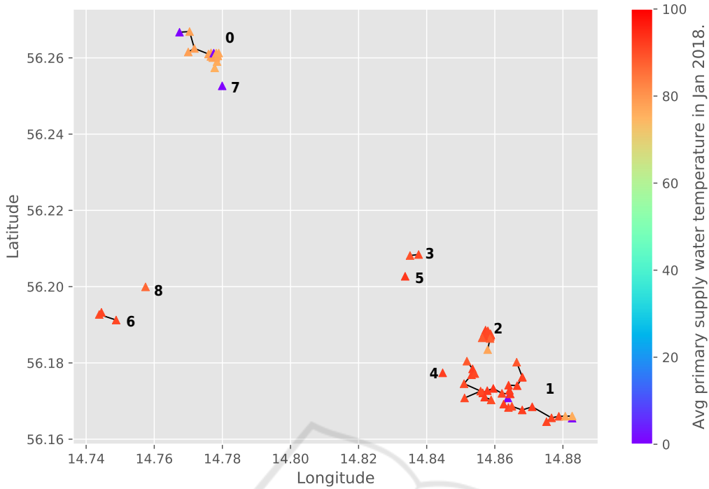
Figure 2: 70 substations located in Southern Sweden are grouped into nine clusters using the MST clustering algorithm. The geographical location of the substations is referred to as the Location view ( v_0 ). Substations with distance less than 500 meters from their closest neighbours are grouped together. The color of the substations represents the average T_{s,1^{st}} in January 2018, which for most substations is around 87 °C.
