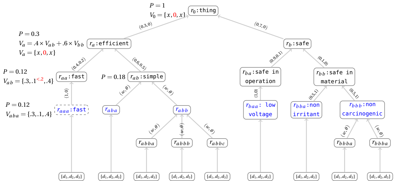
Figure 1: The method ontology structure
